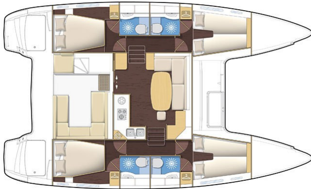
Plan version 4 cabins 4 SBD" / 4 cabins version - 4 washrooms
